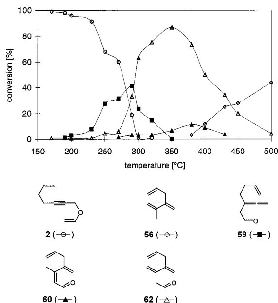
Figure 1. Temperature profile for the pyrolysis of 7-vinylhept-1-en-5-yne ( 2 )
