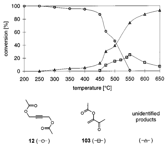
Figure 8. Temperature profile for the pyrolysis of 1,4-bis(acetoxy)-but-2-yne ( 12 )
