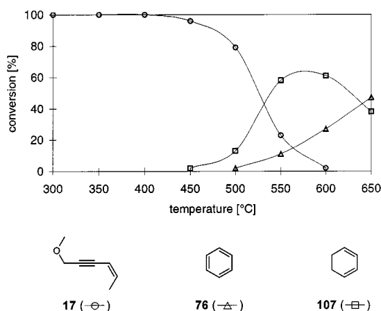
Figure 9. Temperature profile for the pyrolysis of 6-methoxyhex-2-en-4-yne ( 17 )
