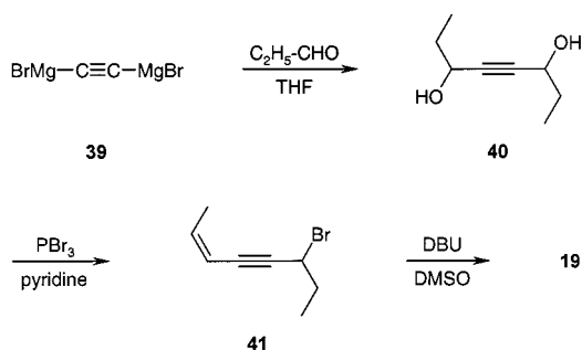
Scheme 7. Preparation of octa-2,6-dien-4-yne ( 19 )
