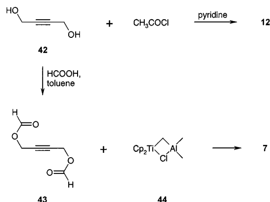
Scheme 8. Preparation of the diester 12 and the divinyl ether 7
