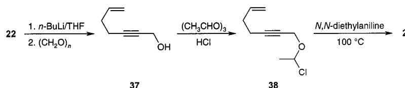
Scheme 6. Preparation of the unsymmetrical propargyl vinyl ether 2
