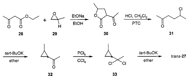
Scheme 3. Preparation of trans -1-ethynyl-2-methylcyclopropane ( trans - 27 )
