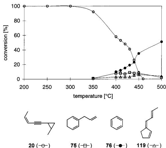
Figure 12. Temperature profile for the pyrolysis of 5-(2-methylcyclopropyl)pent-2-en-4-yne ( 20 )
