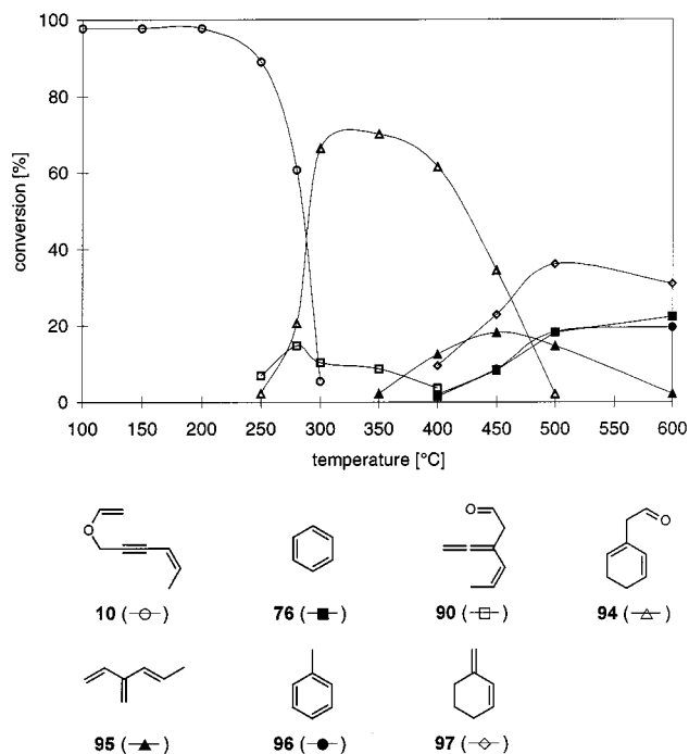
Figure 7. Temperature profile for the pyrolysis of 6-vinyloxyhex-2-en-4-yne ( 10 )
