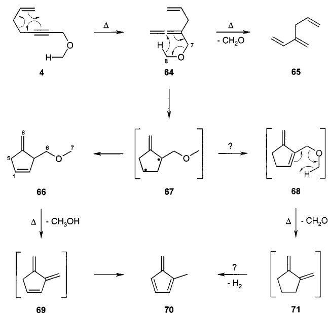
Scheme 11. Tandem pericyclic processes in the pyrolysis of 4
