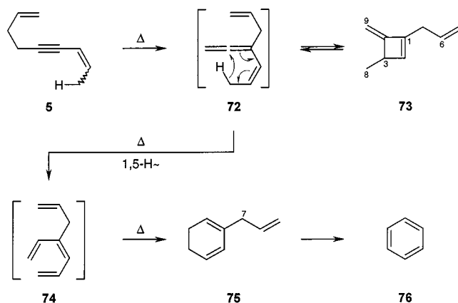
Scheme 12. Tandem pericyclic processes in the pyrolysis of 5
