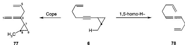
Scheme 13. Tandem pericyclic processes in the pyrolysis of 6
