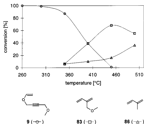
Figure 6. Temperature profile for the pyrolysis of 1-methoxy-4-vinyloxybut-2-yne ( 9 )
