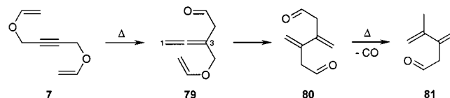
Scheme 14. Tandem pericyclic processes in the pyrolysis of 7
