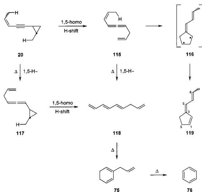
Scheme 20. Tandem pericyclic processes in the pyrolysis of 20
