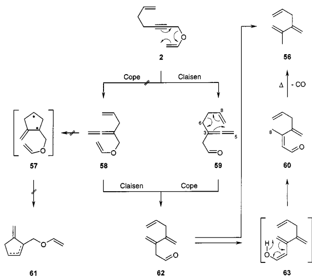
Scheme 10. Tandem pericyclic processes in the pyrolysis of 2
