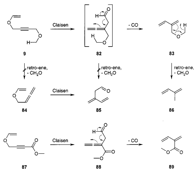
Scheme 15. Tandem pericyclic processes in the pyrolysis of 9
