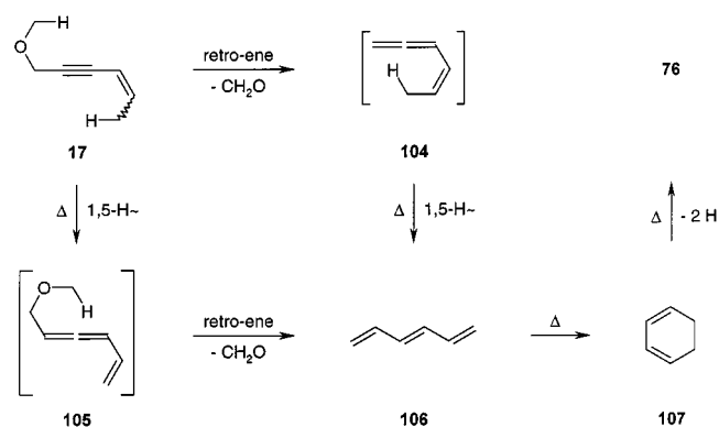
Scheme 18. Tandem pericyclic processes in the pyrolysis of 17
