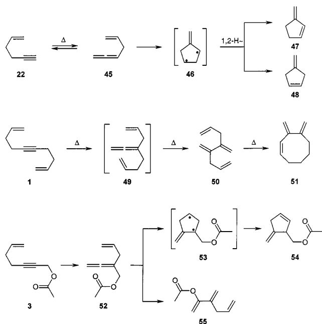
Scheme 9. Tandem pericyclic reactions of 1 and 3
