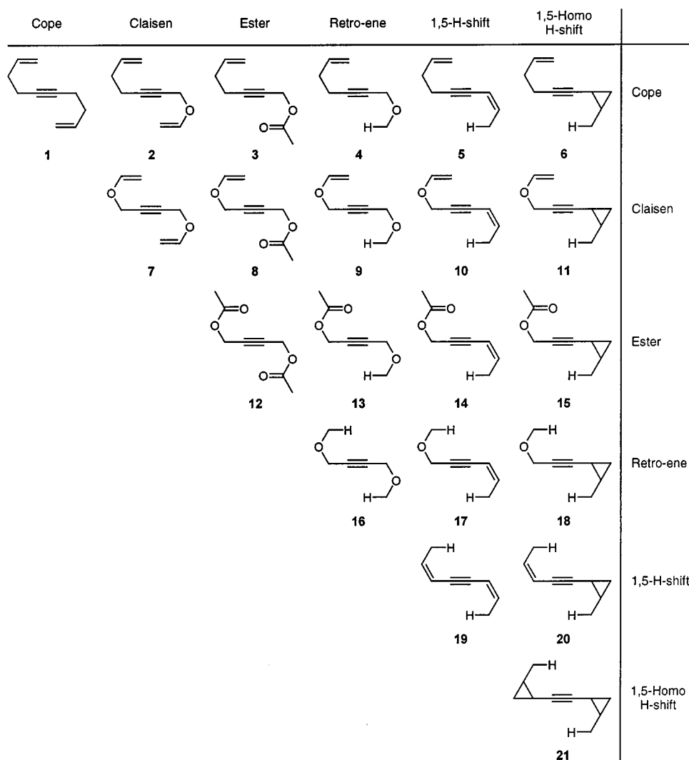
Scheme 1. A selection of substrates for tandem reactions involving disubstituted alkynes
