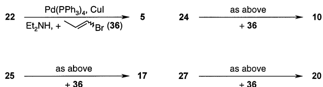
Scheme 5. Preparation of the conjugated enynes 5 , 10 , 17 , and 20
