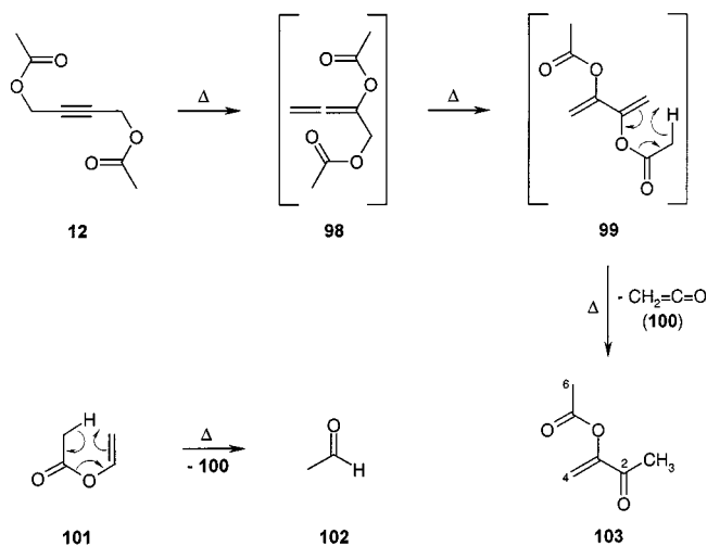
Scheme 17. Tandem pericyclic processes in the pyrolysis of 12
