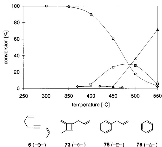
Figure 3. Temperature profile for the pyrolysis of nona-1,7-dien-5-yne ( 5 )
