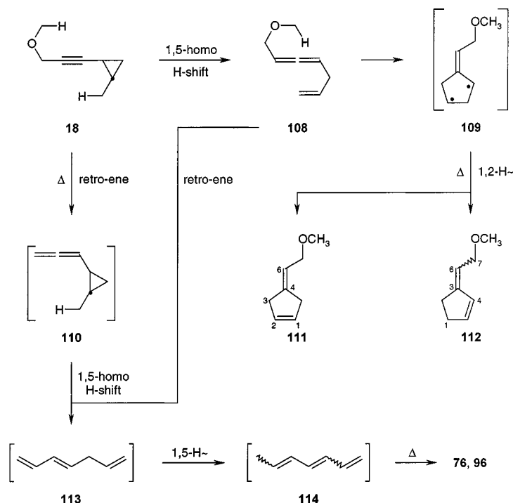
Scheme 19. Tandem pericyclic processes in the pyrolysis of 18
