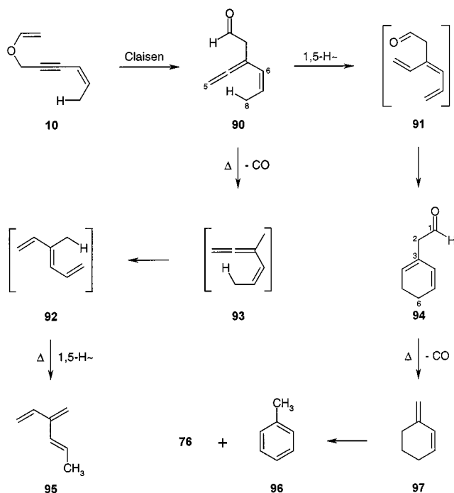
Scheme 16. Tandem pericyclic processes in the pyrolysis of 10
