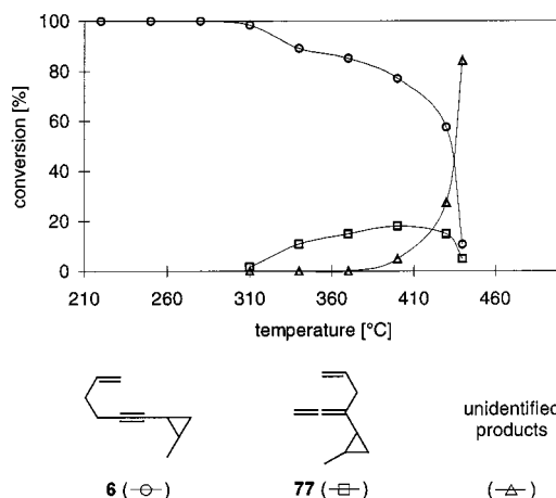
Figure 4. Temperature profile for the pyrolysis of 1-(hex-5-en-1-ynyl)-2-methylcyclopropane ( 6 )
