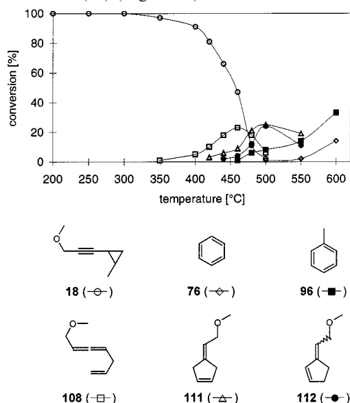
Figure 10. Temperature profile for the pyrolysis of 1-(3-methoxyprop-1-ynyl)-2-methylcyclopropane ( 18 )
