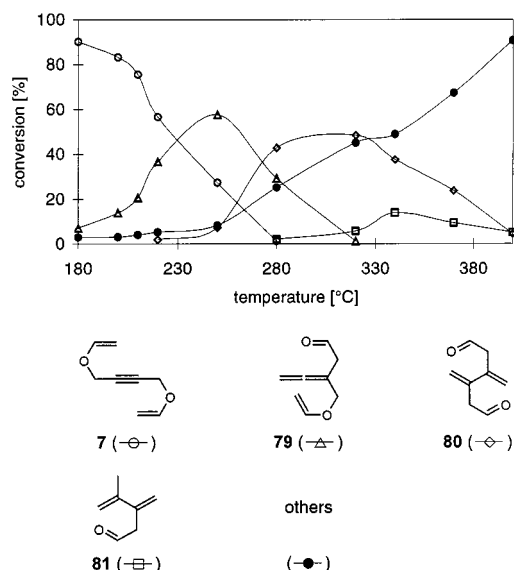
Figure 5. Temperature profile for the pyrolysis of 1,4-bis(vinyloxy)but-2-yne ( 7 )
