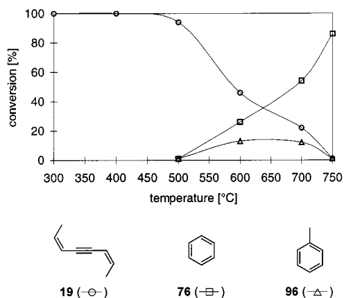
Figure 11. Temperature profile for the pyrolysis of octa-2,6-dien-4-yne ( 19 )
